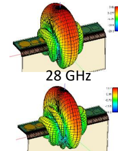
Array Realized Gain
